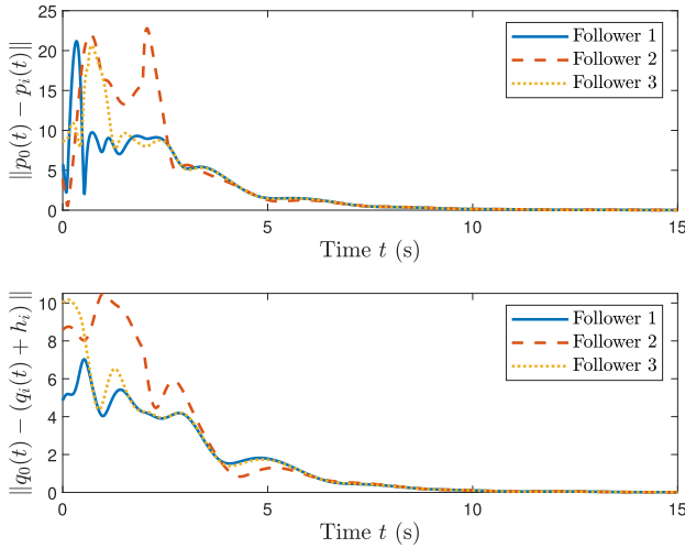
Fig. 1. Velocity and position tracking errors of followers.
